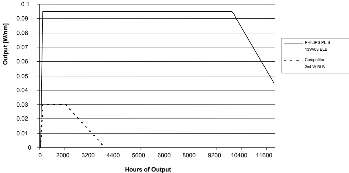
Comparison of PL-S 13W/08 and Competitors 2x4 W BLB
